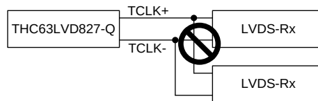
Figure 14. Multi Drop Connection
