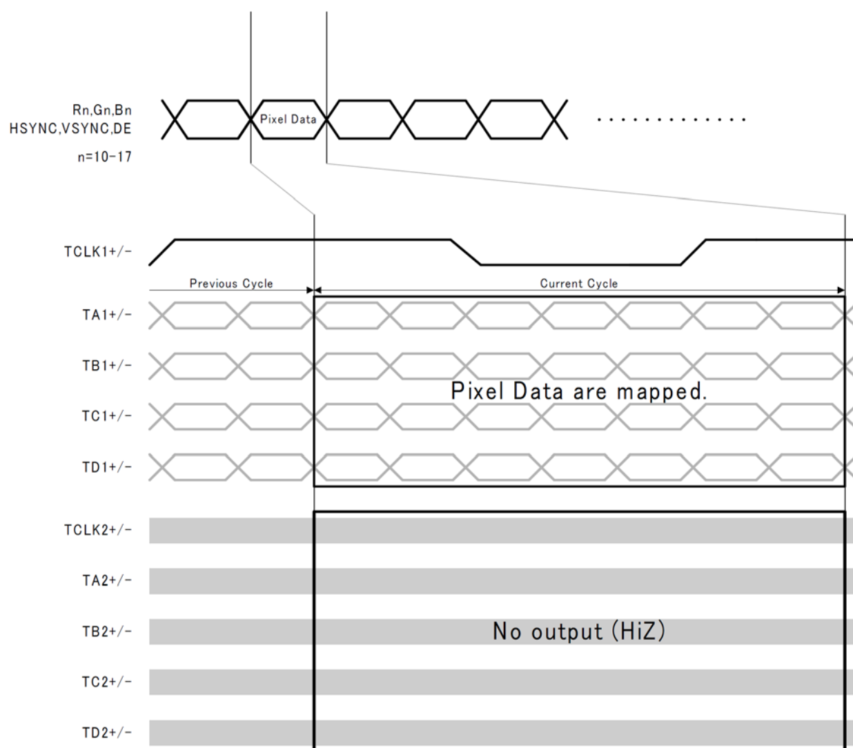
Figure 11. Single-In / Single-Out Mode (MODE = H)
